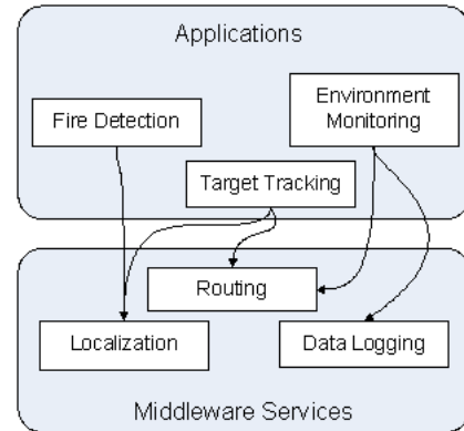
Figure 1. Middleware services are shared among concurrently executing applications, resulting in a many-to-many relationship between applications and services.
