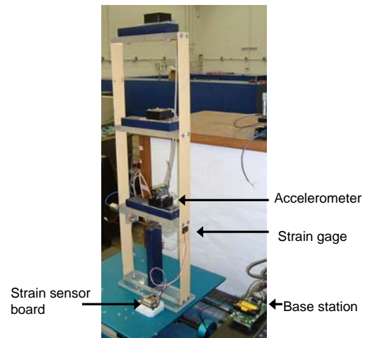
Figure 5. Experiment setup.
