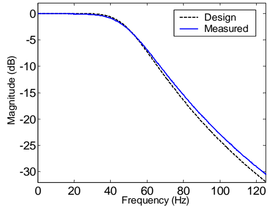
Figure 3. Anti-aliasing filter transfer function.
